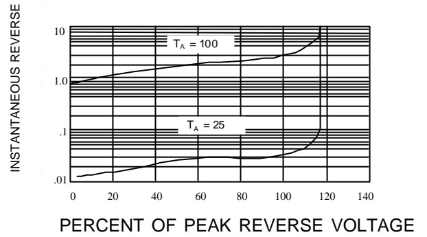
Fig. 4-TYPICAL REVERSE CHARACTERISTICS
