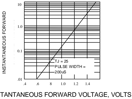
Fig. 3-TYPICAL FORWARD CHARACTERISTICS
